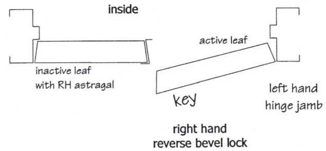
Right hand reverse active (RHRA) (out swing)
