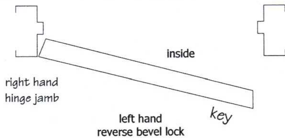
Left hand reverse (LHR) (out swing)
