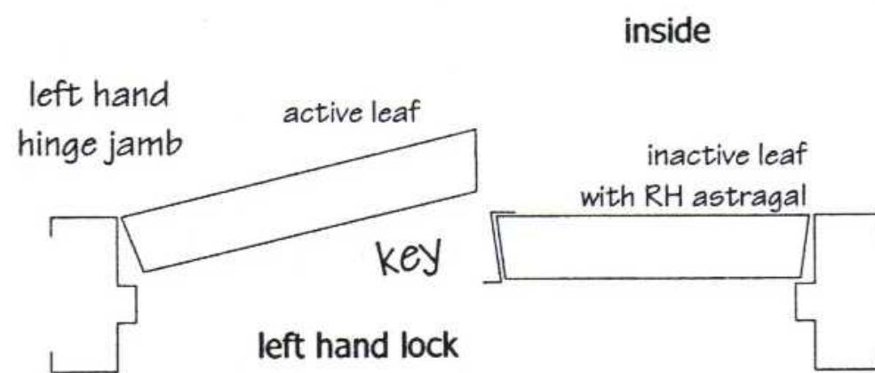
Left hand active (LHA) (in swing)
