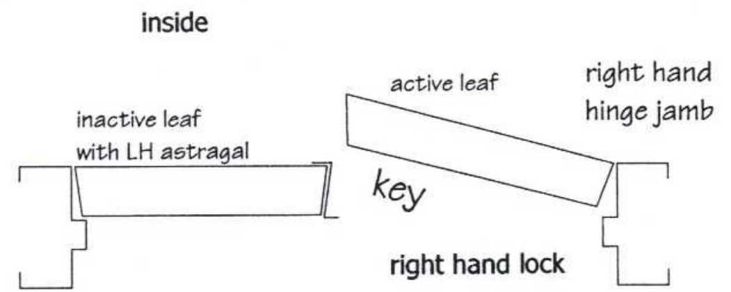
Right hand active (RHA) (in swing)
