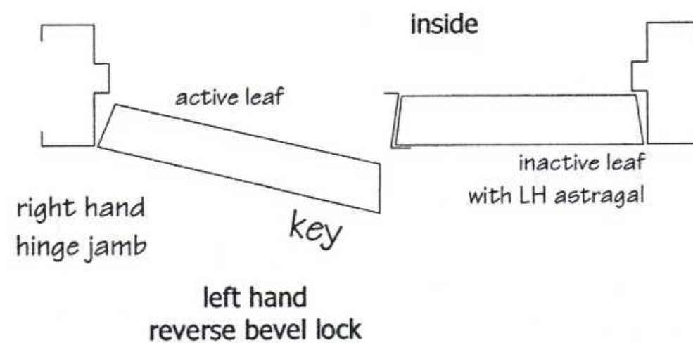
Left hand reverse active (LHRA) (out swing)
